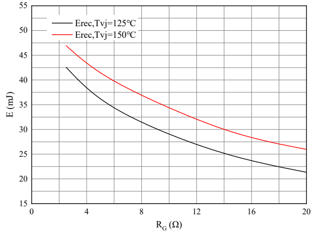
图 8. 开关损耗 二极管 Figure 8. Switching losses of Diode IF=300A, V CE =900V
