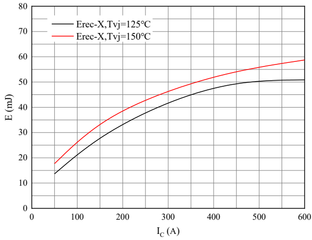
图 7. 开关损耗 二极管 Figure 7. Switching losses of Diode R Gon =2.5 Ω, V CE =900V
